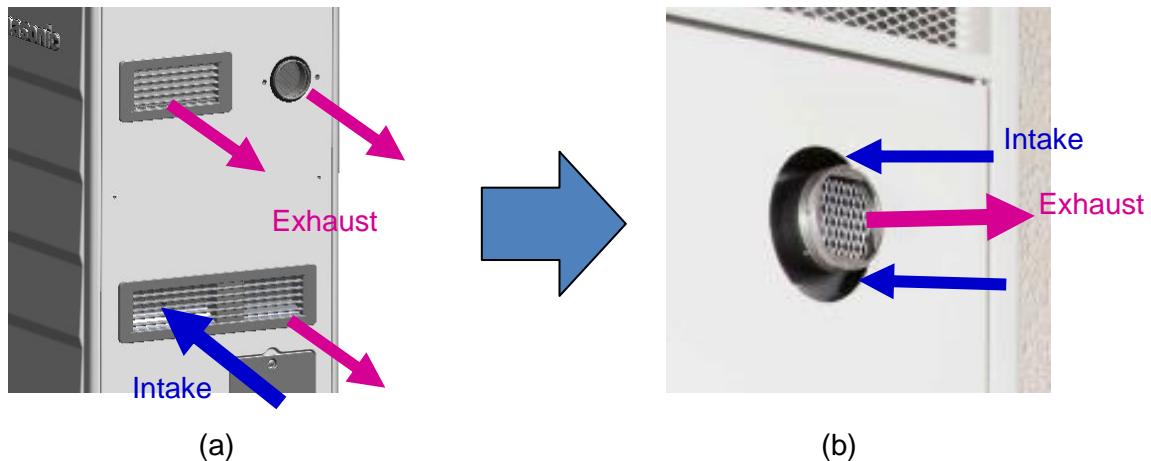
Fig 8: Construction of intake/exhaust: (a) conventional model, and (b) apartment houses model
