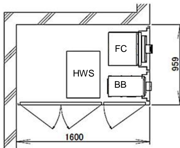
Fig 7: An Example of installation layout of ENE-FARM installed in a pipe shaft
