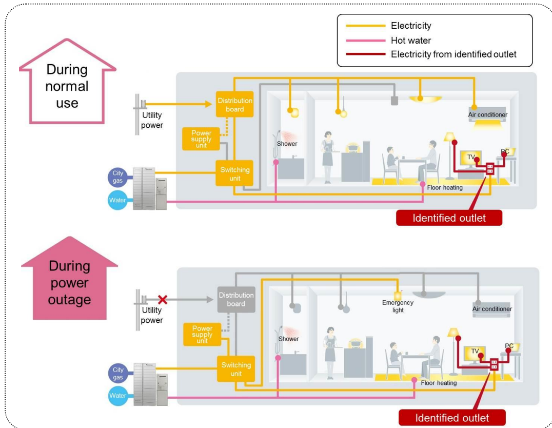
Fig 10: Flow of electricity of Option B
