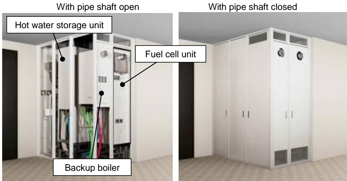
Fig 2: Image of ENE-FARM installed in a pipe shaft of apartment buildings
