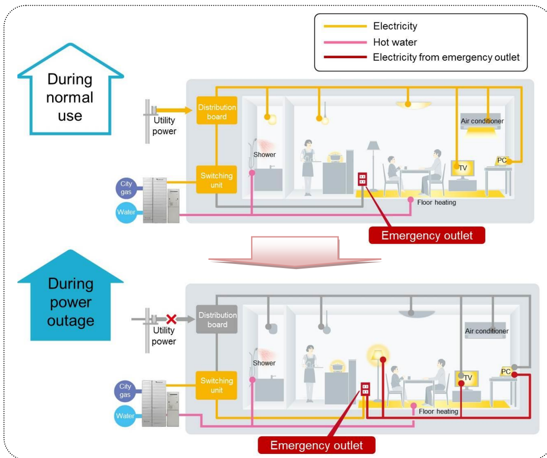
Fig 9: Flow of electricity of Option A
